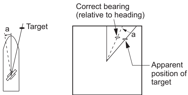
Antenna mounted error to port (HDG SW advanced) Picture appears deviated clockwise.
