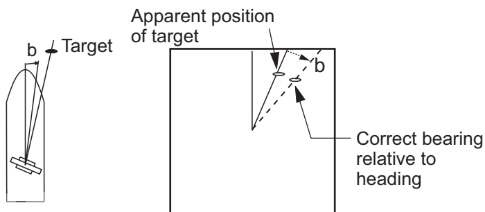
Antenna mounted error to port (HDG SW delayed) Picture appears deviated counterclockwise.
