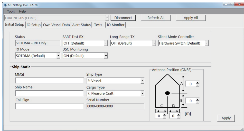
[Status] ([AIS Status] on the external display), [Serial Number]: Display only.
