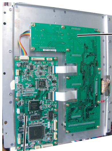
05P0859 T-CPU
