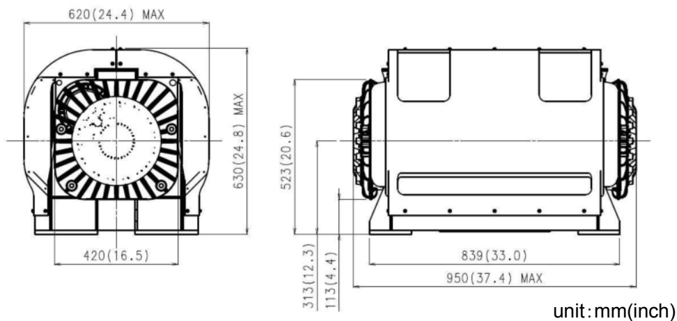
Figure 2-5 Dimensions for the ARG unit
