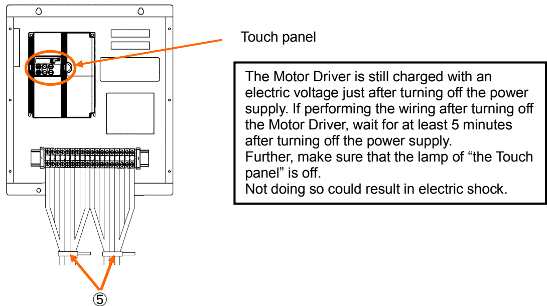
Figure 4-16 How to check the electric voltage just after turned off the Motor Driver
