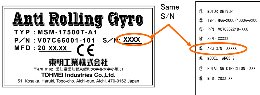
Figure 4-8 Combination of the ARG unit and Motor Driver
