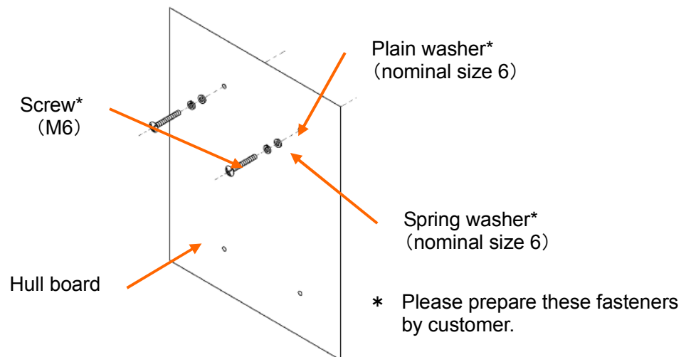
Figure 4-9 Procedure 1 for Motor Driver installation
