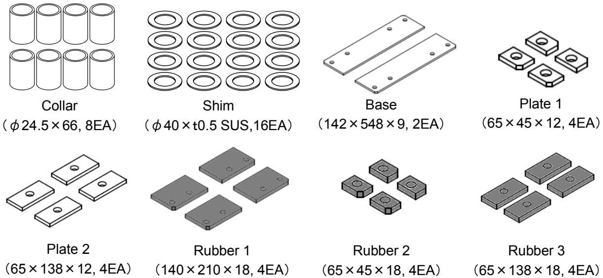
Figure 2-2 Checking of the delivered ARG (No.2)
